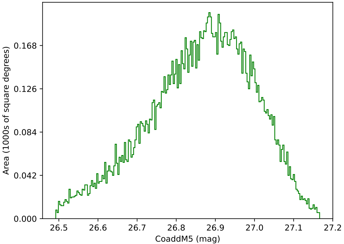
too_elab_r8_d3_giz_v3.4_10yrs WFD g band: CoaddM5
