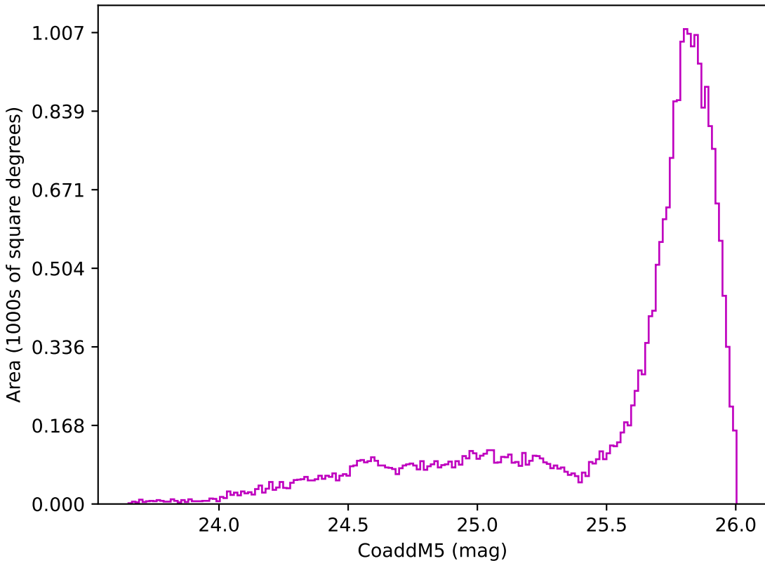
too_elab_r8_d3_giz_v3.4_10yrs All sky z band: CoaddM5
