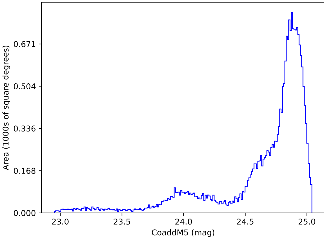
too_elab_r8_d3_giz_v3.4_10yrs All sky y band: CoaddM5
