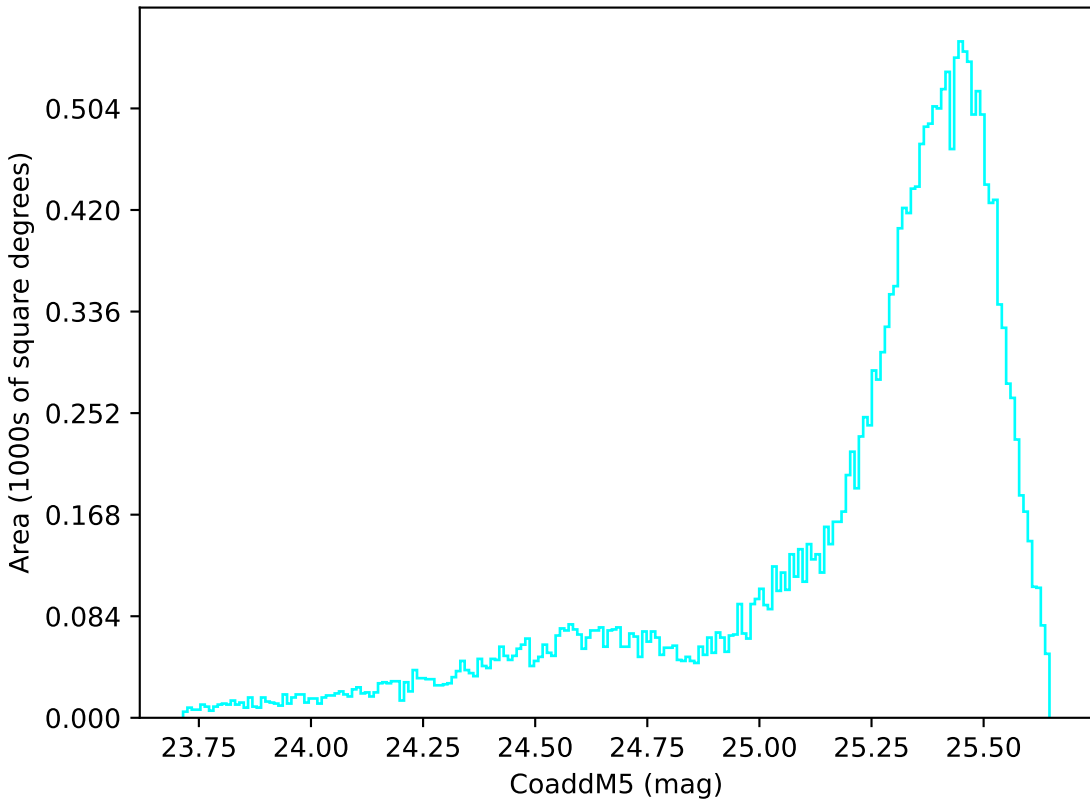
too_elab_r8_d3_giz_v3.4_10yrs All sky u band: CoaddM5
