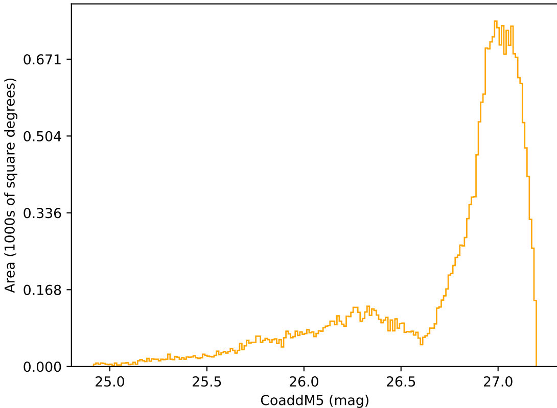
too_elab_r8_d3_giz_v3.4_10yrs All sky r band: CoaddM5
