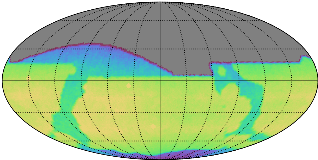
too_elab_r8_d3_giz_v3.4_10yrs All sky i band: CoaddM5
