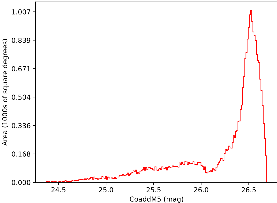
too_elab_r8_d3_giz_v3.4_10yrs All sky i band: CoaddM5
