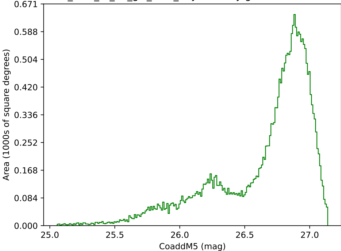
too_elab_r8_d3_giz_v3.4_10yrs All sky g band: CoaddM5
