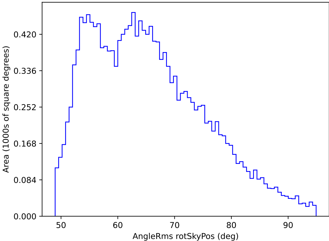
too_elab_r8_d3_giz_v3.4_10yrs WFD z band: AngleRms rotSkyPos
