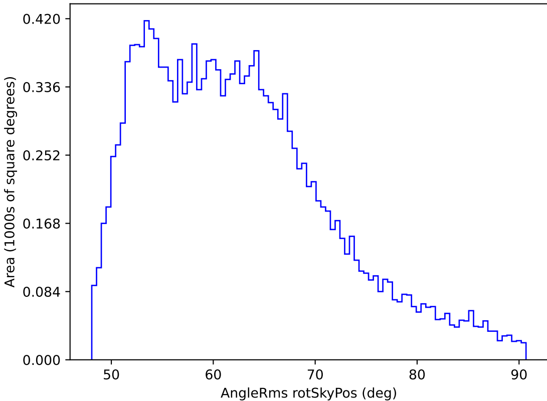
too_elab_r8_d3_giz_v3.4_10yrs WFD y band: AngleRms rotSkyPos
