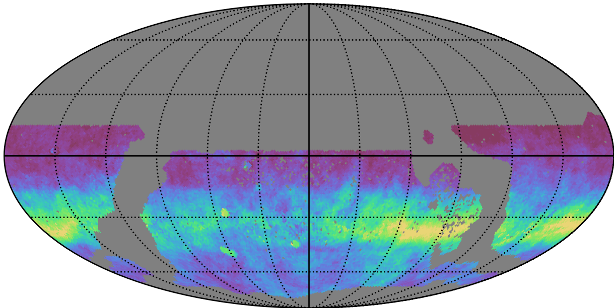
too_elab_r8_d3_giz_v3.4_10yrs WFD r band: AngleRms rotSkyPos
