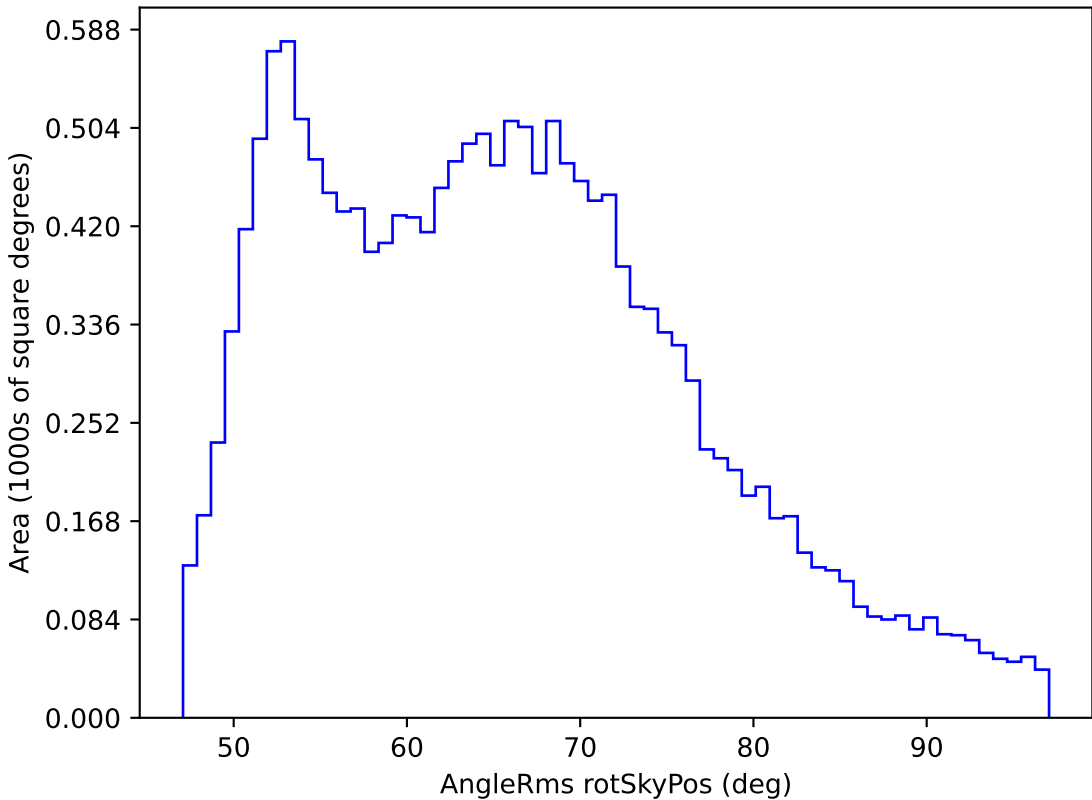
too_elab_r8_d3_giz_v3.4_10yrs WFD r band: AngleRms rotSkyPos
