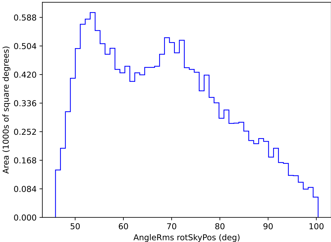
too_elab_r8_d3_giz_v3.4_10yrs WFD g band: AngleRms rotSkyPos
