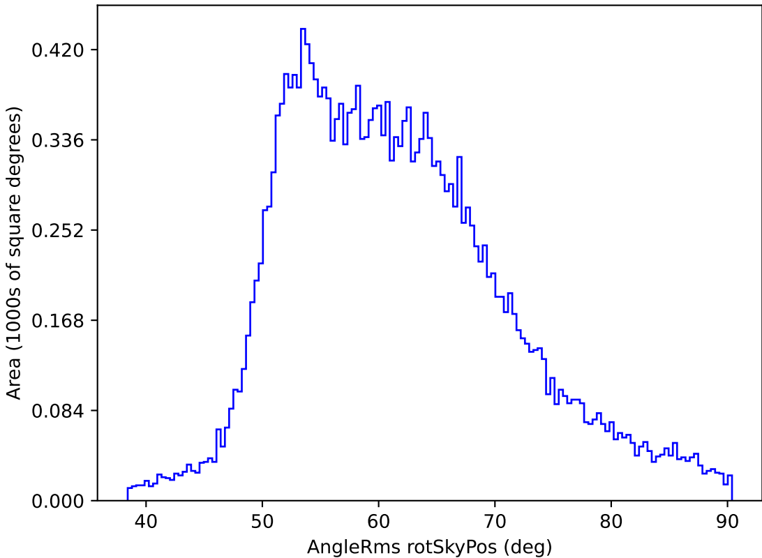
too_elab_r8_d3_giz_v3.4_10yrs All sky y band: AngleRms rotSkyPos
