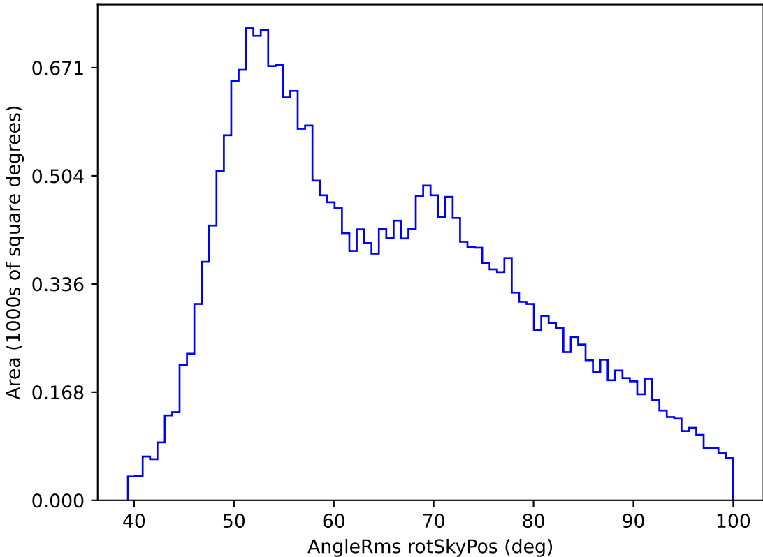
too_elab_r8_d3_giz_v3.4_10yrs All sky g band: AngleRms rotSkyPos
