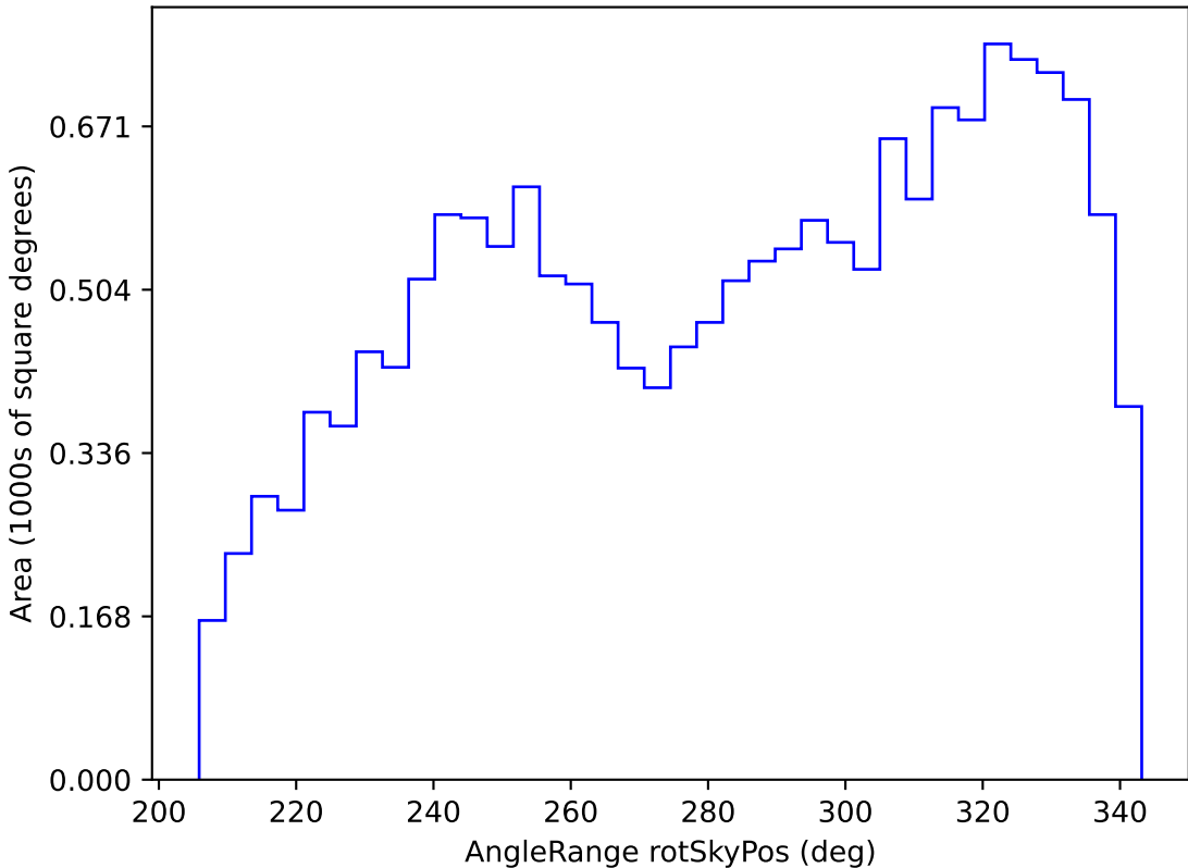
too_elab_r8_d3_giz_v3.4_10yrs WFD z band: AngleRange rotSkyPos
