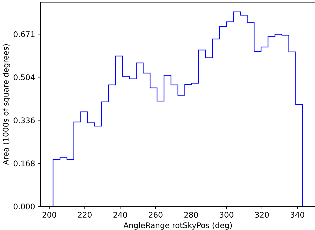
too_elab_r8_d3_giz_v3.4_10yrs WFD r band: AngleRange rotSkyPos
