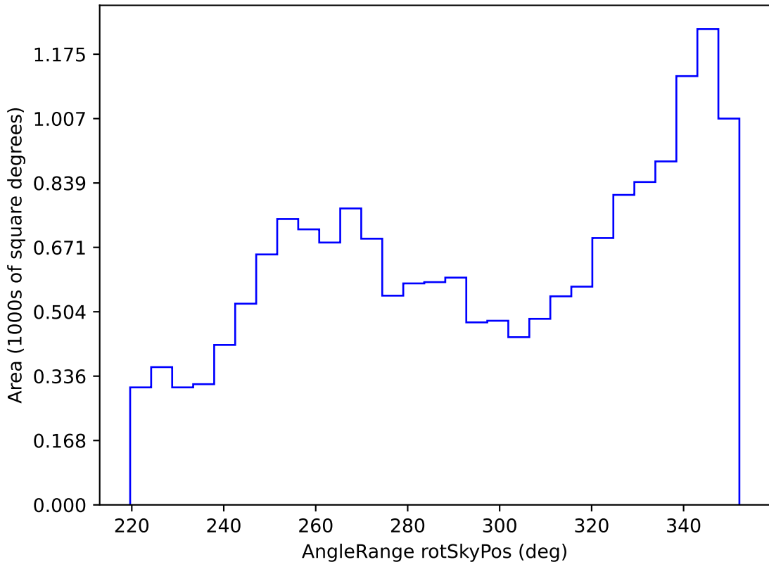
too_elab_r8_d3_giz_v3.4_10yrs WFD all bands: AngleRange rotSkyPos
