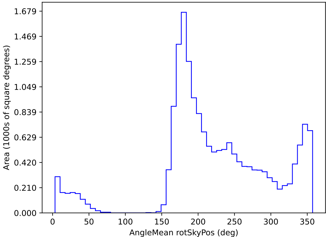
too_elab_r8_d3_giz_v3.4_10yrs WFD u band: AngleMean rotSkyPos
