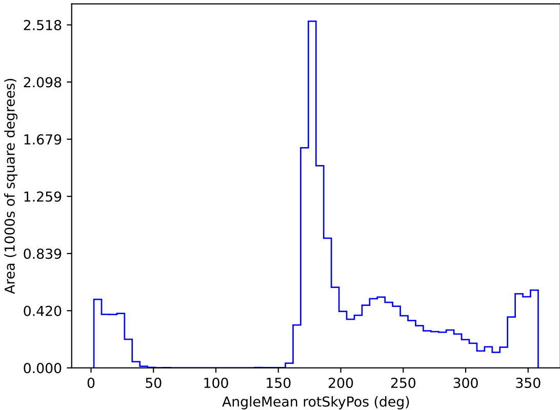
too_elab_r8_d3_giz_v3.4_10yrs WFD r band: AngleMean rotSkyPos
