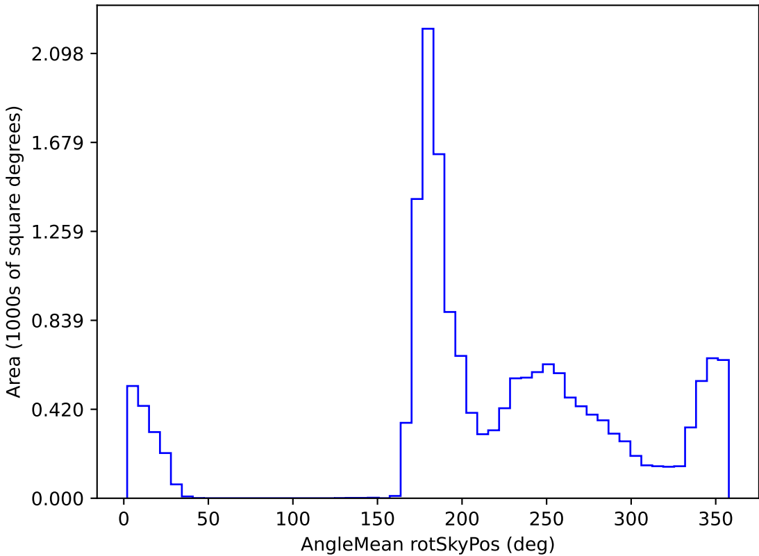
too_elab_r8_d3_giz_v3.4_10yrs WFD i band: AngleMean rotSkyPos
