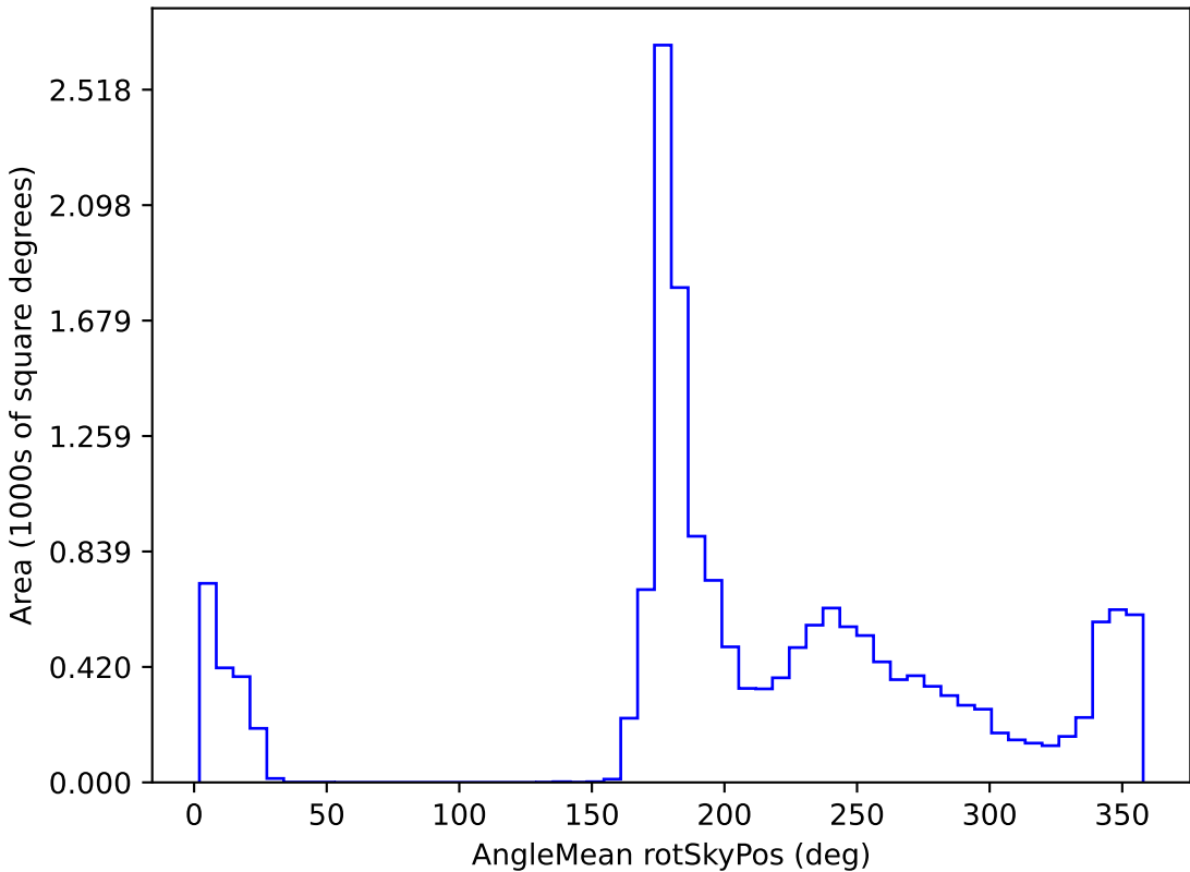
too_elab_r8_d3_giz_v3.4_10yrs WFD all bands: AngleMean rotSkyPos
