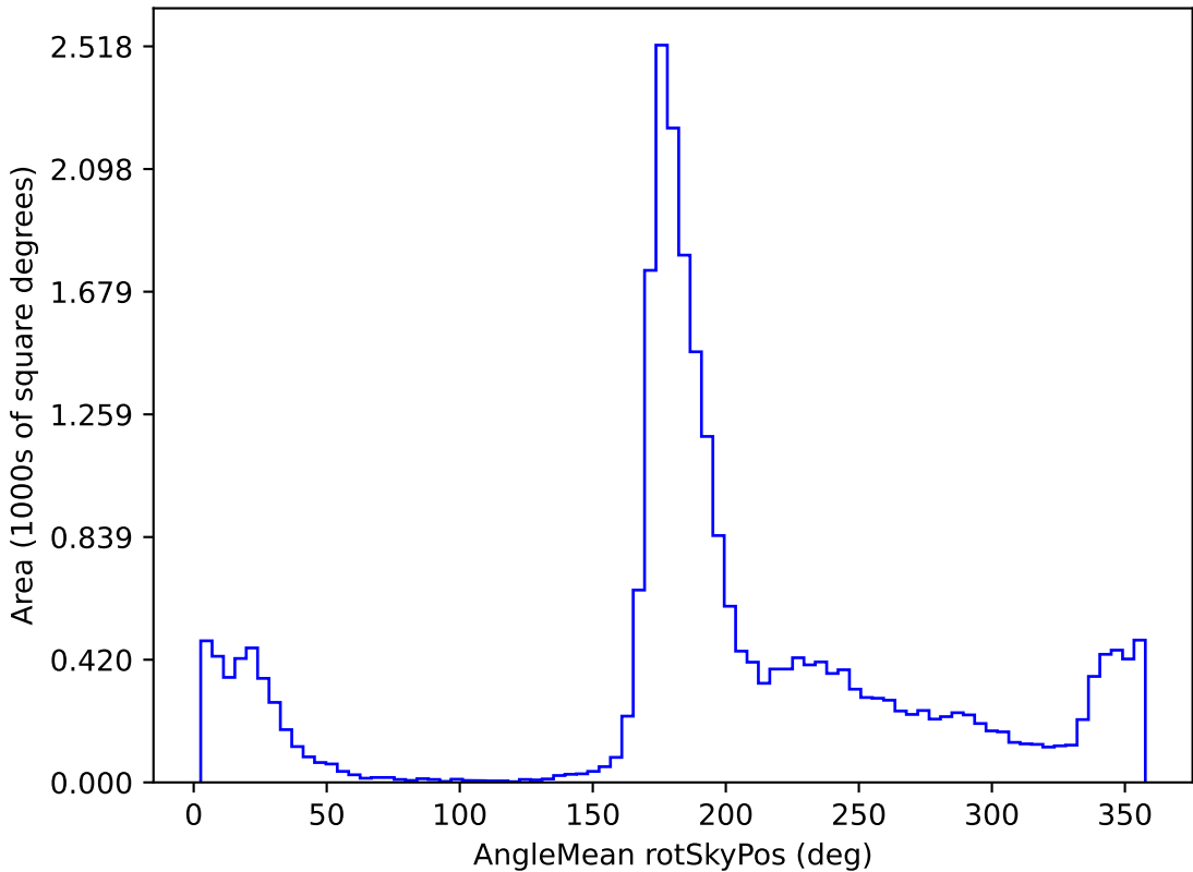
too_elab_r8_d3_giz_v3.4_10yrs All sky r band: AngleMean rotSkyPos
