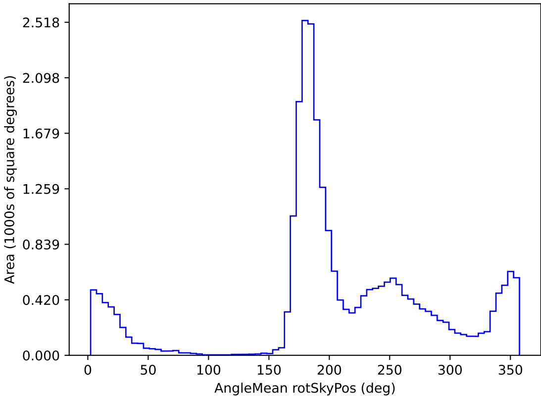
too_elab_r8_d3_giz_v3.4_10yrs All sky i band: AngleMean rotSkyPos
