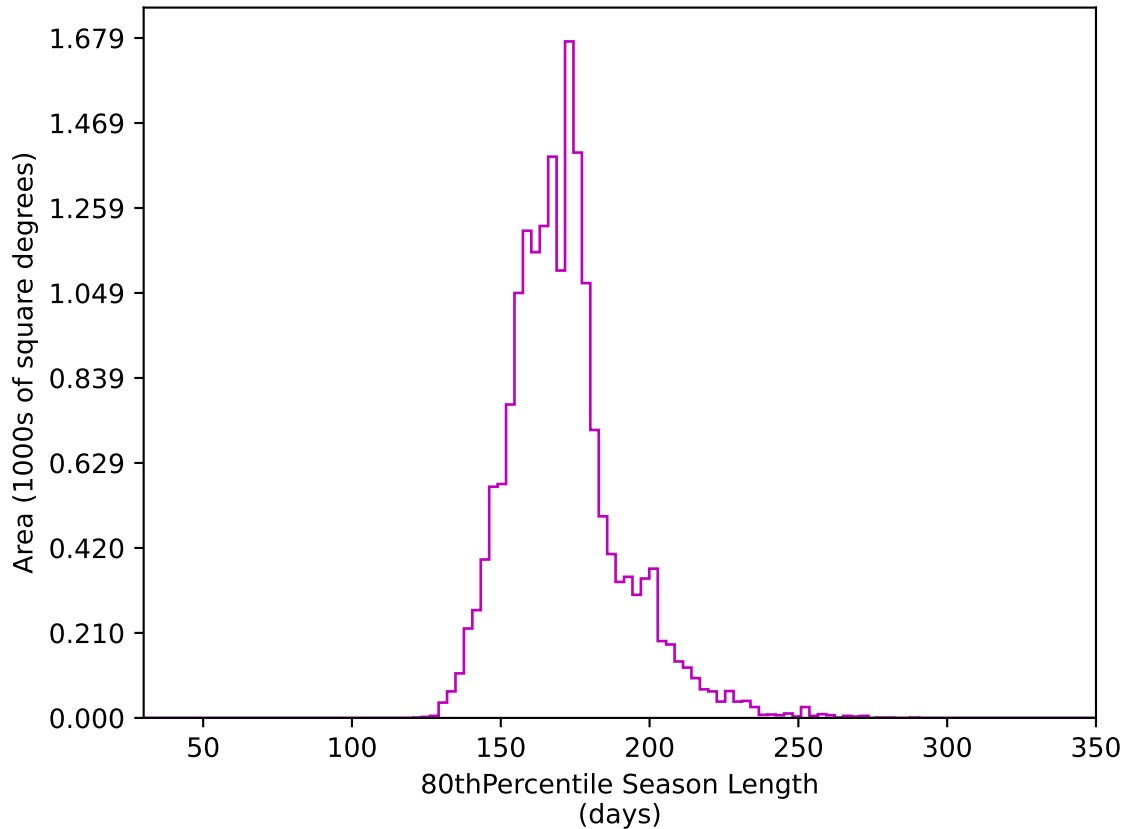
too_elab_r8_d3_giz_v3.4_10yrs WFD z band: 80thPercentile Season Length
