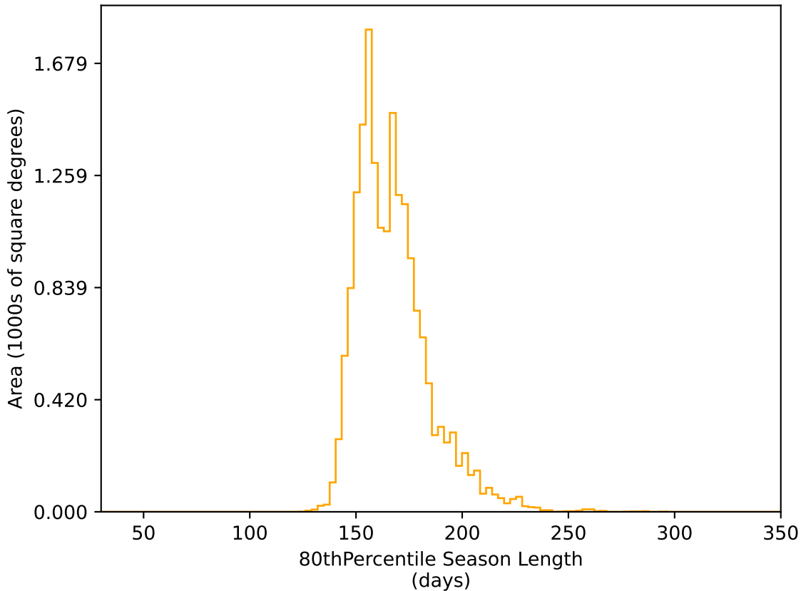
too_elab_r8_d3_giz_v3.4_10yrs WFD r band: 80thPercentile Season Length
