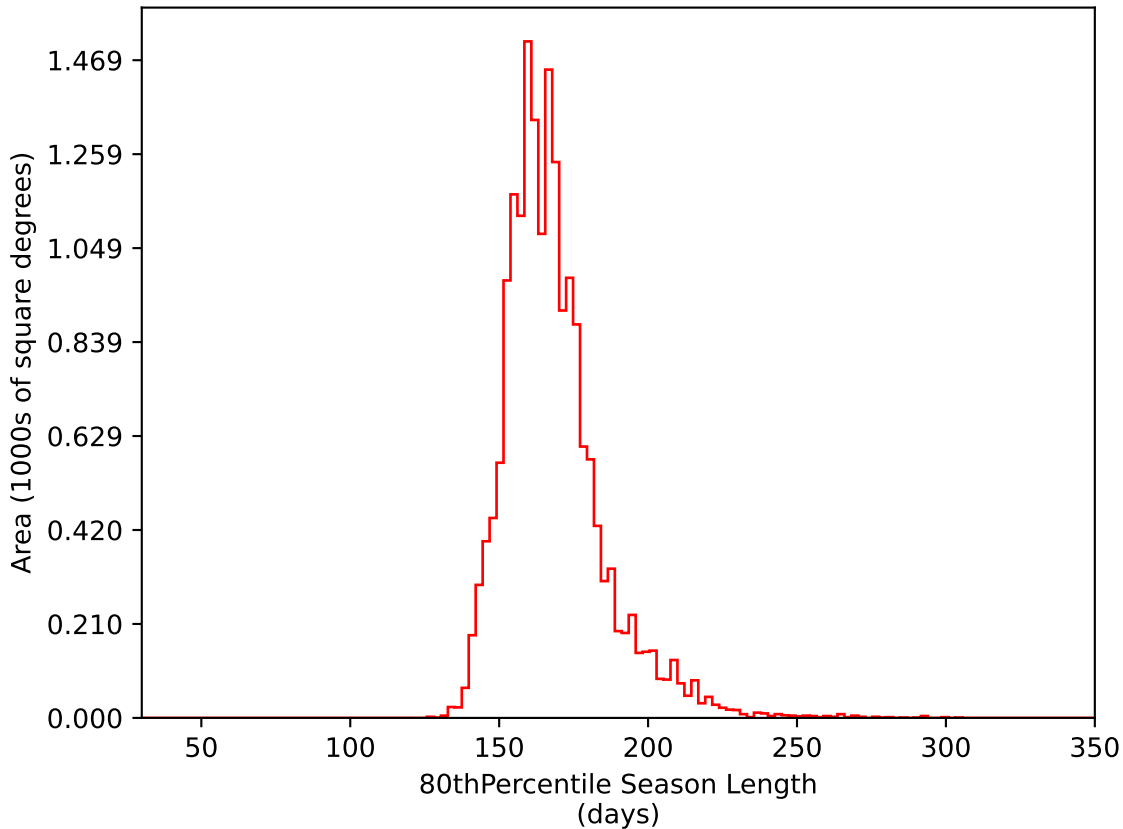
too_elab_r8_d3_giz_v3.4_10yrs WFD i band: 80thPercentile Season Length
