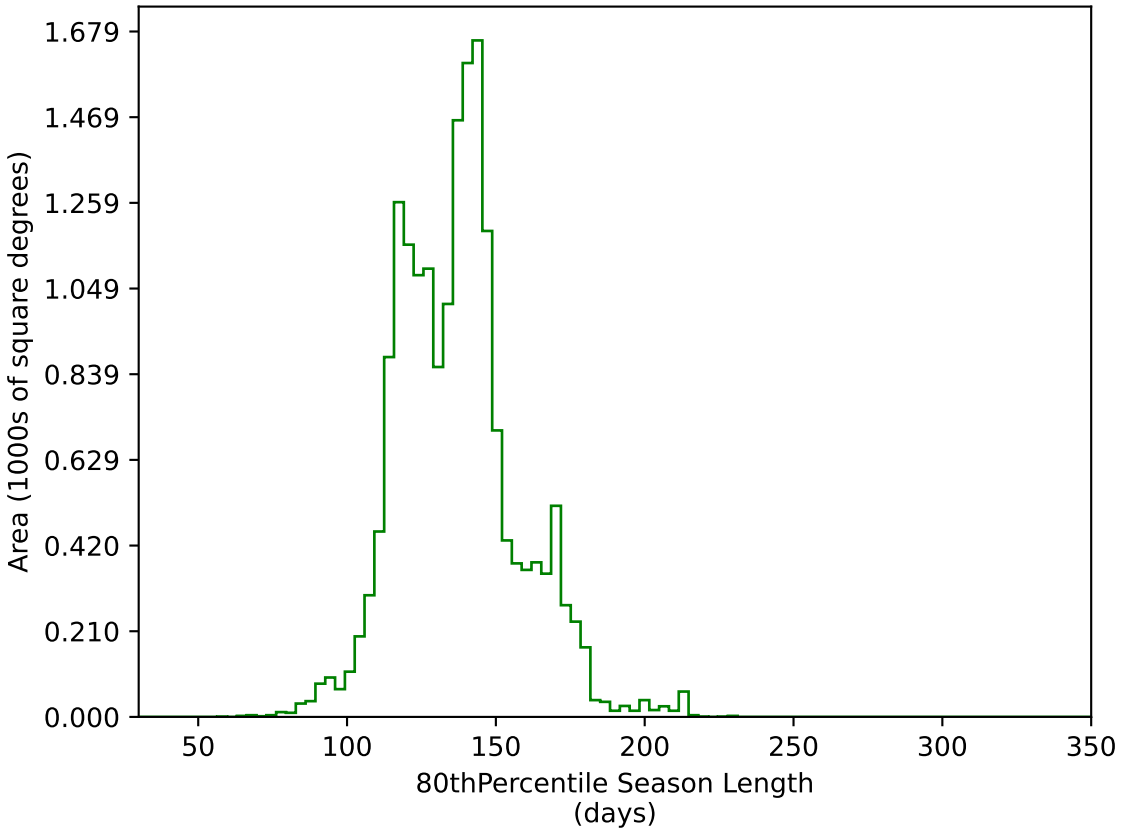
too_elab_r8_d3_giz_v3.4_10yrs WFD g band: 80thPercentile Season Length
