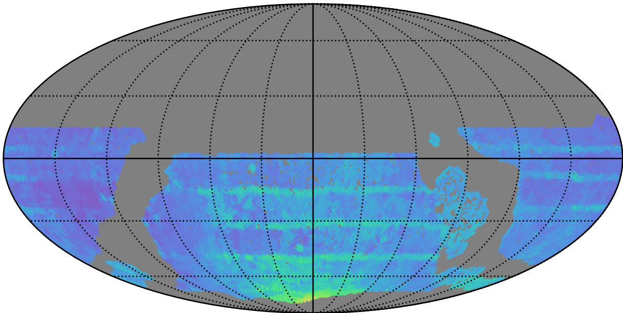
too_elab_r8_d3_giz_v3.4_10yrs WFD all bands: 80thPercentile Season Length
