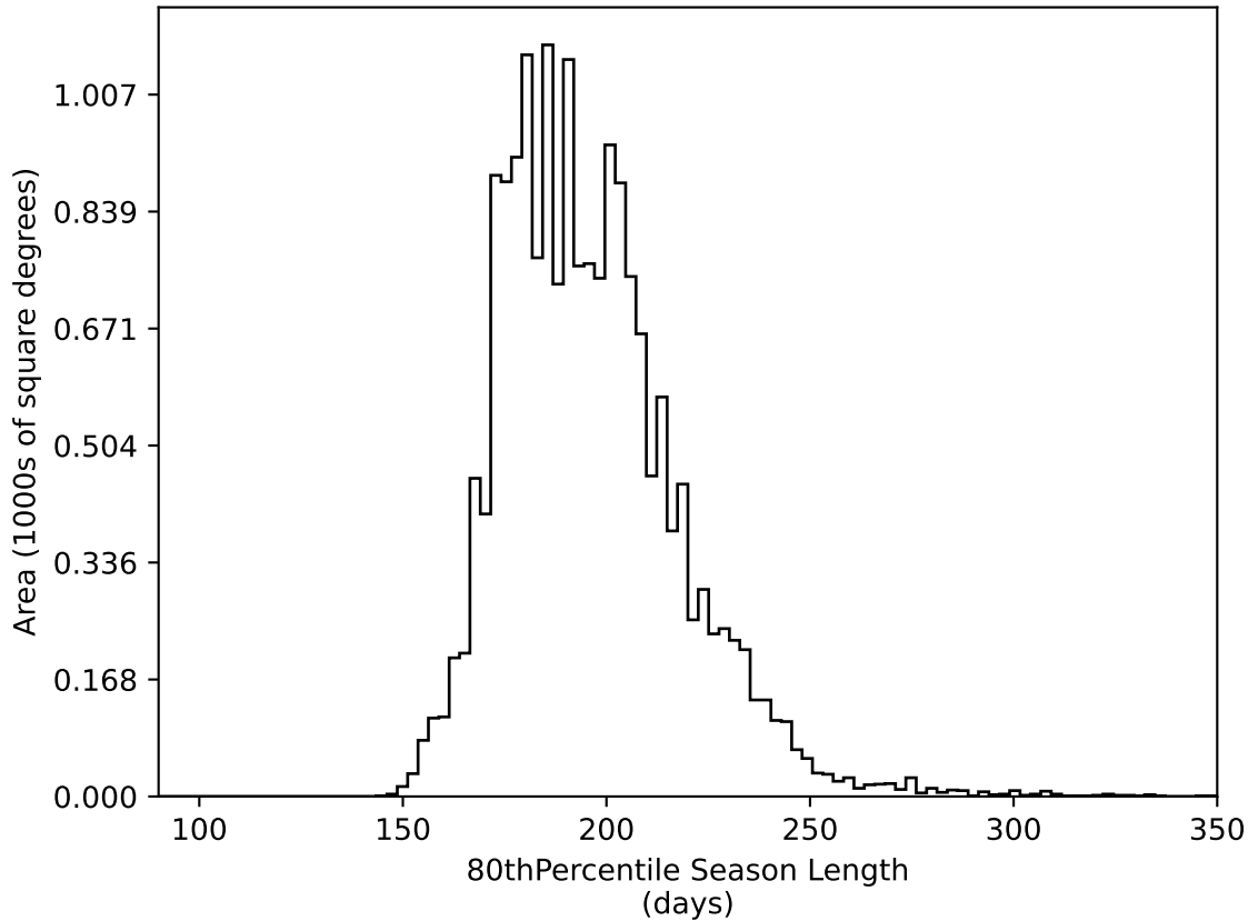
too_elab_r8_d3_giz_v3.4_10yrs WFD all bands: 80thPercentile Season Length
