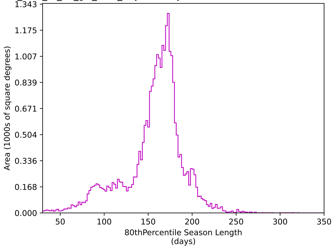
too_elab_r8_d3_giz_v3.4_10yrs All sky z band: 80thPercentile Season Length
