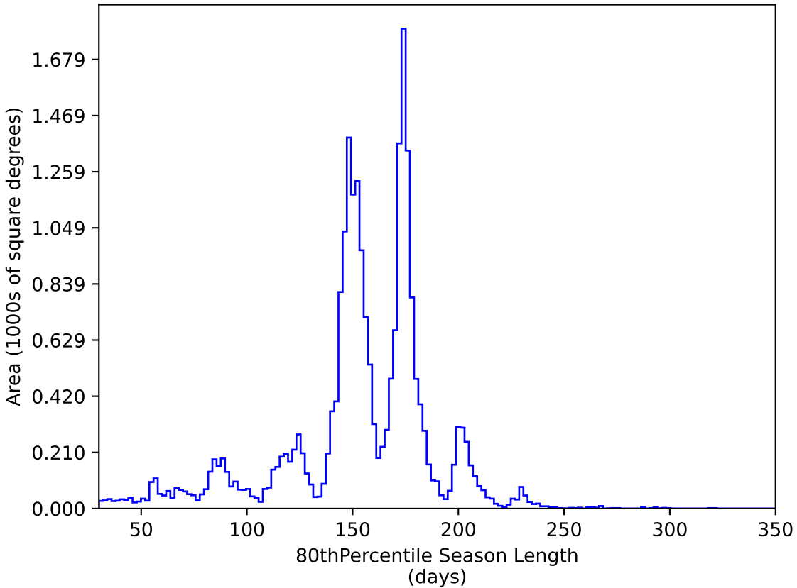
too_elab_r8_d3_giz_v3.4_10yrs All sky y band: 80thPercentile Season Length
