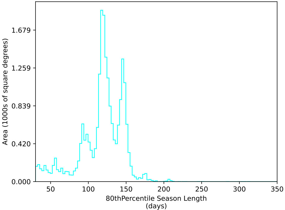
too_elab_r8_d3_giz_v3.4_10yrs All sky u band: 80thPercentile Season Length
