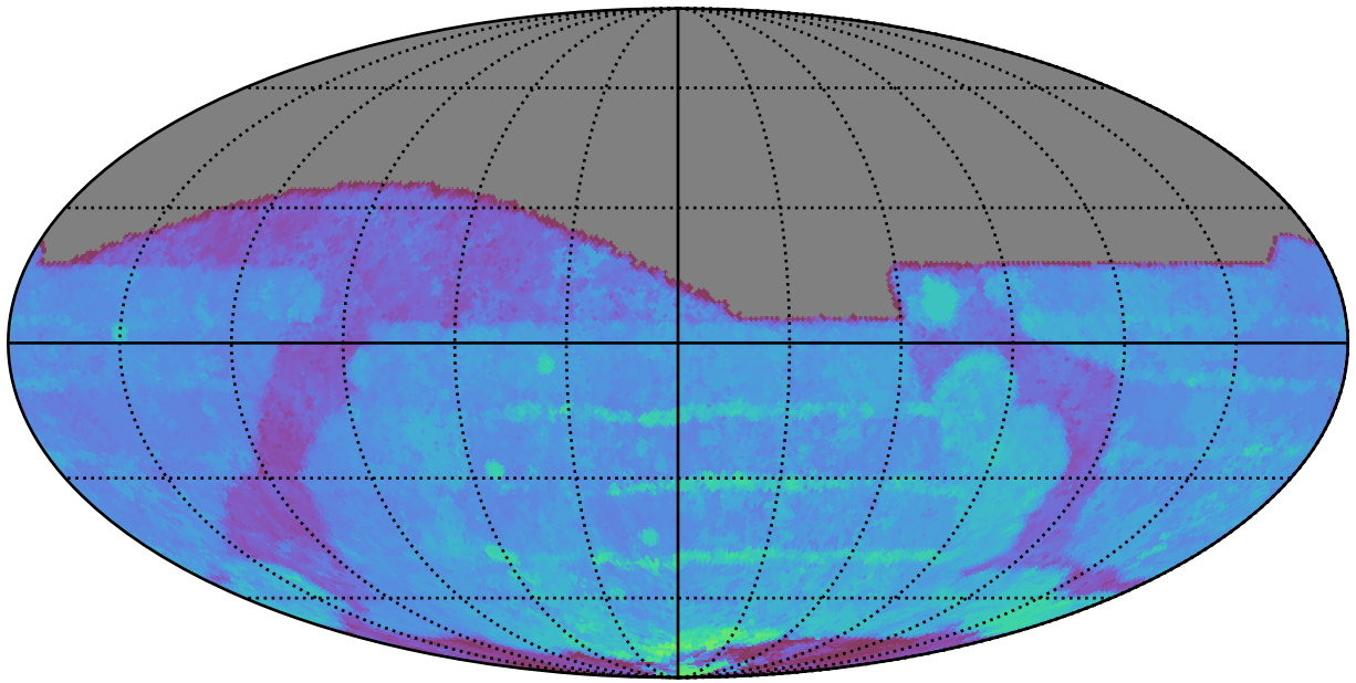
too_elab_r8_d3_giz_v3.4_10yrs All sky r band: 80thPercentile Season Length
