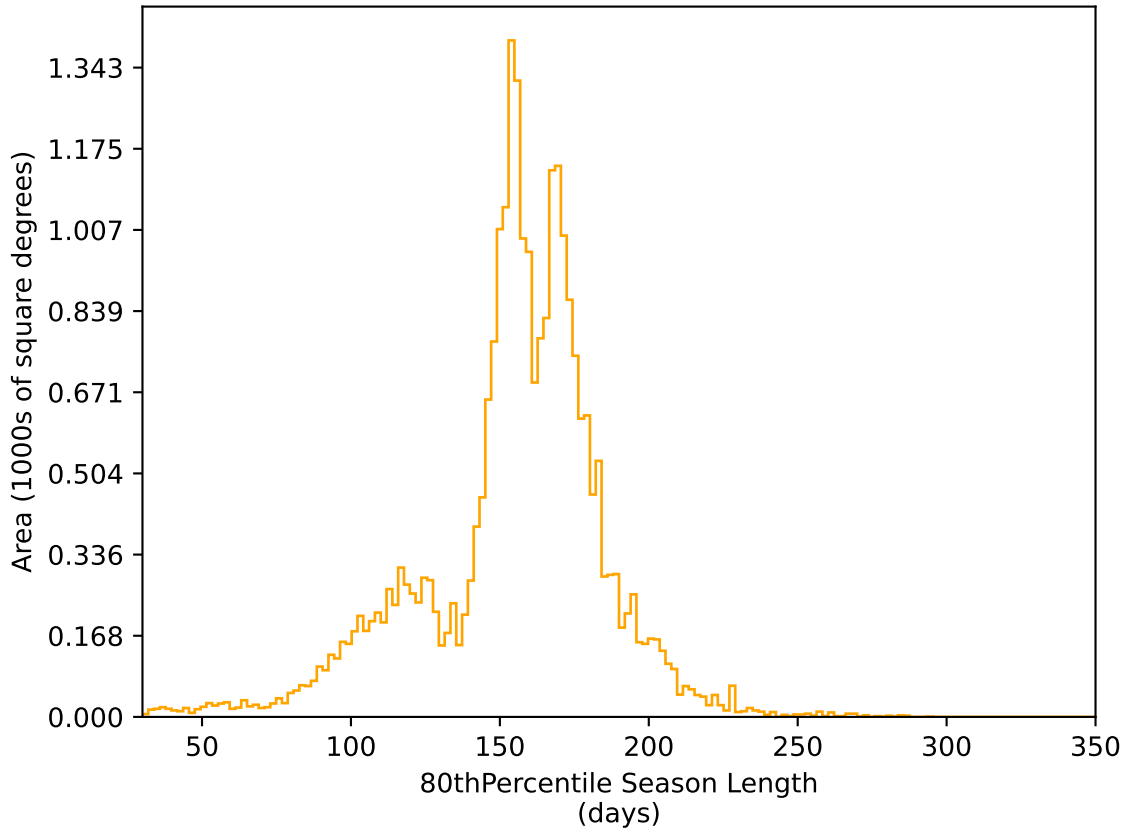
too_elab_r8_d3_giz_v3.4_10yrs All sky r band: 80thPercentile Season Length
