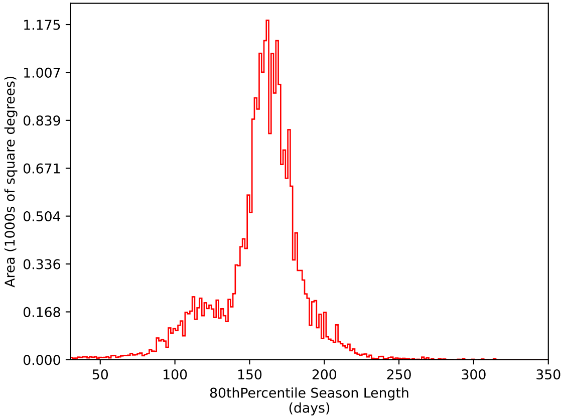
too_elab_r8_d3_giz_v3.4_10yrs All sky i band: 80thPercentile Season Length
