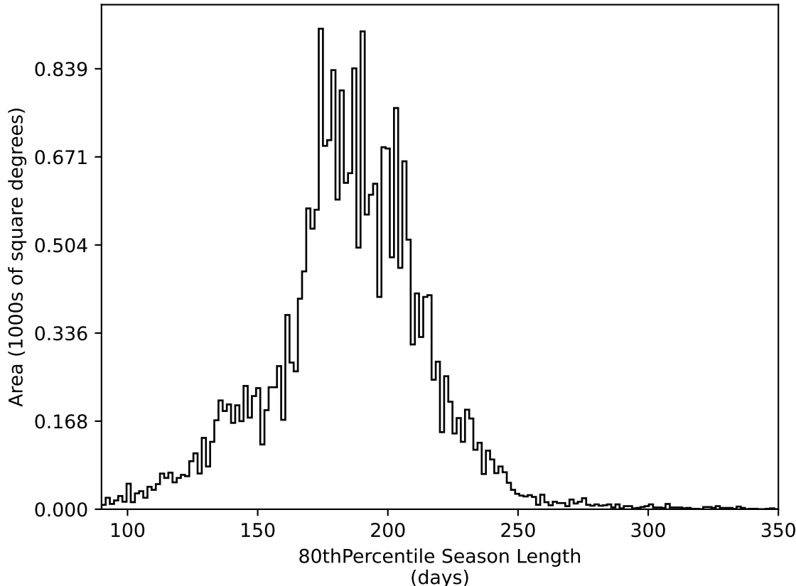
too_elab_r8_d3_giz_v3.4_10yrs All sky all bands: 80thPercentile Season Length
