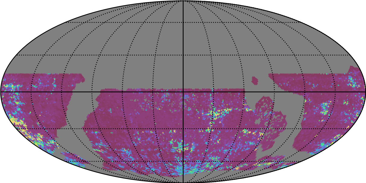
too_elab_r8_d3_giz_v3.4_10yrs WFD z band: 75th Percentile Intranight Timespan
