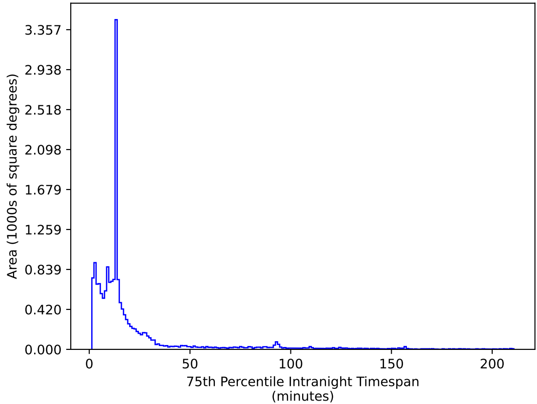
too_elab_r8_d3_giz_v3.4_10yrs WFD z band: 75th Percentile Intranight Timespan
