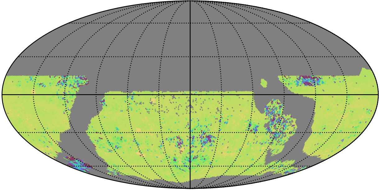
too_elab_r8_d3_giz_v3.4_10yrs WFD ug bands: 75th Percentile Intranight Timespan
