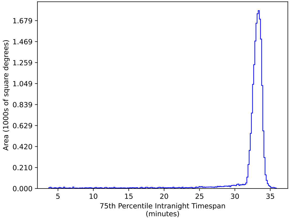
too_elab_r8_d3_giz_v3.4_10yrs WFD ug bands: 75th Percentile Intranight Timespan
