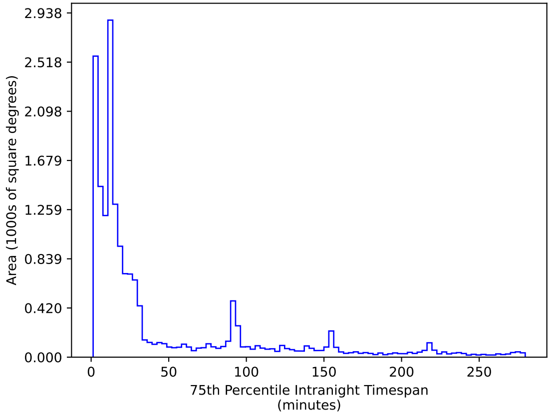
too_elab_r8_d3_giz_v3.4_10yrs WFD r band: 75th Percentile Intranight Timespan
