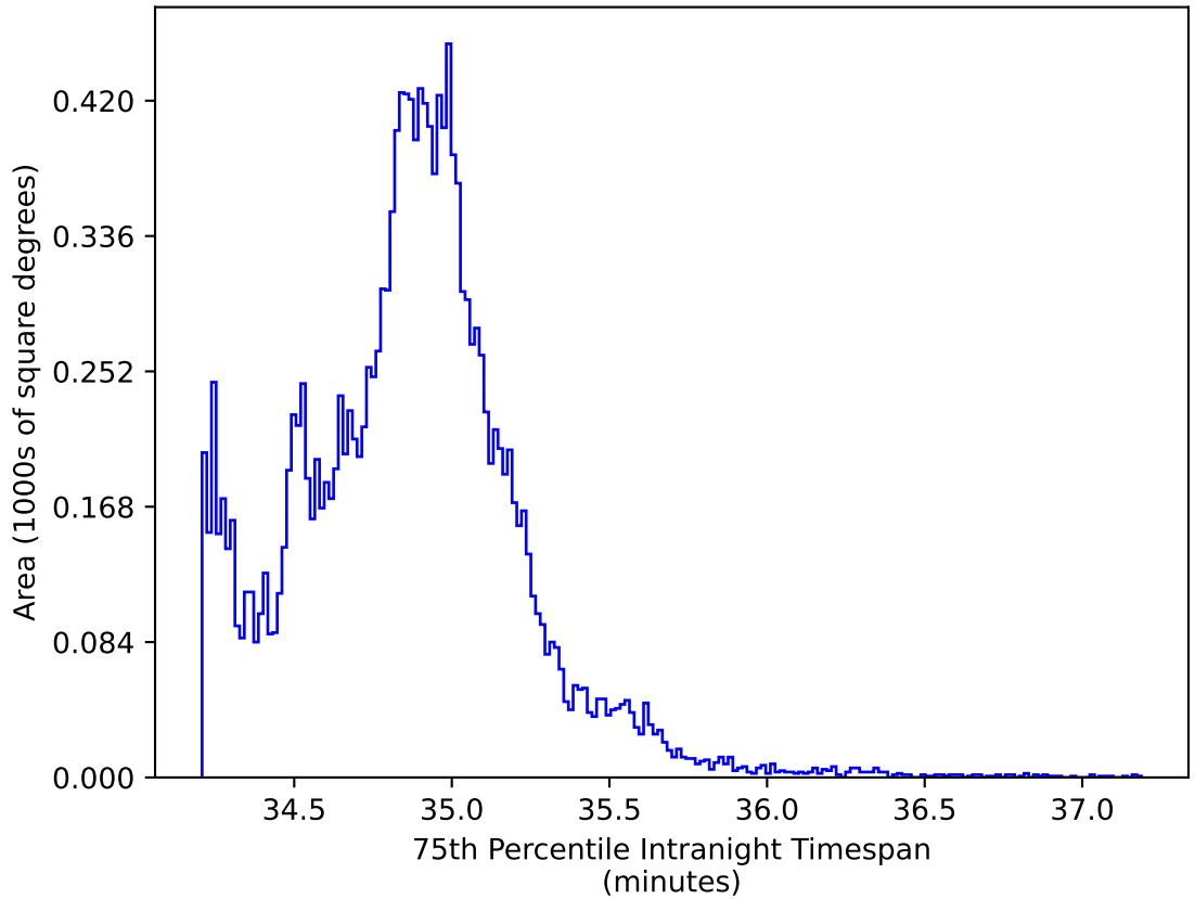
too_elab_r8_d3_giz_v3.4_10yrs WFD iz bands: 75th Percentile Intranight Timespan
