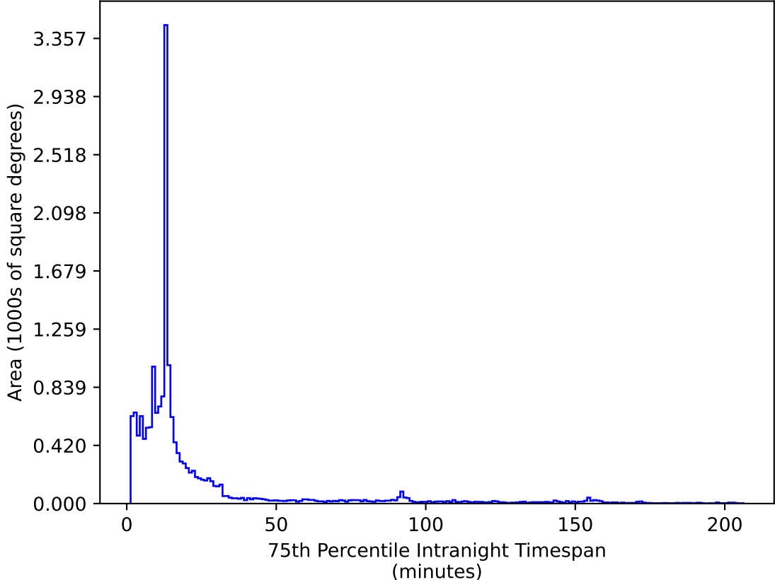
too_elab_r8_d3_giz_v3.4_10yrs WFD i band: 75th Percentile Intranight Timespan
