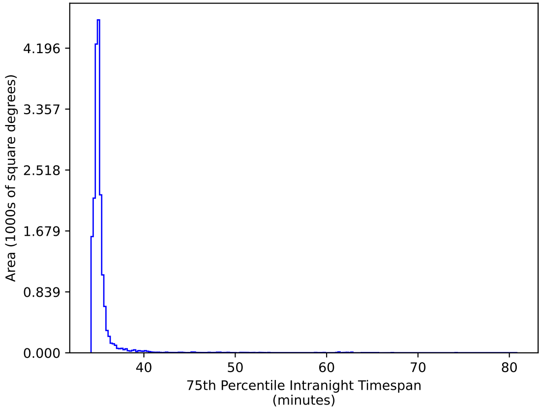
too_elab_r8_d3_giz_v3.4_10yrs WFD gr bands: 75th Percentile Intranight Timespan
