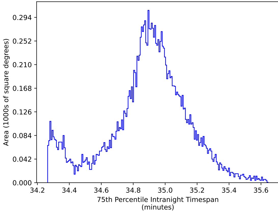
too_elab_r8_d3_giz_v3.4_10yrs WFD all bands: 75th Percentile Intranight Timespan
