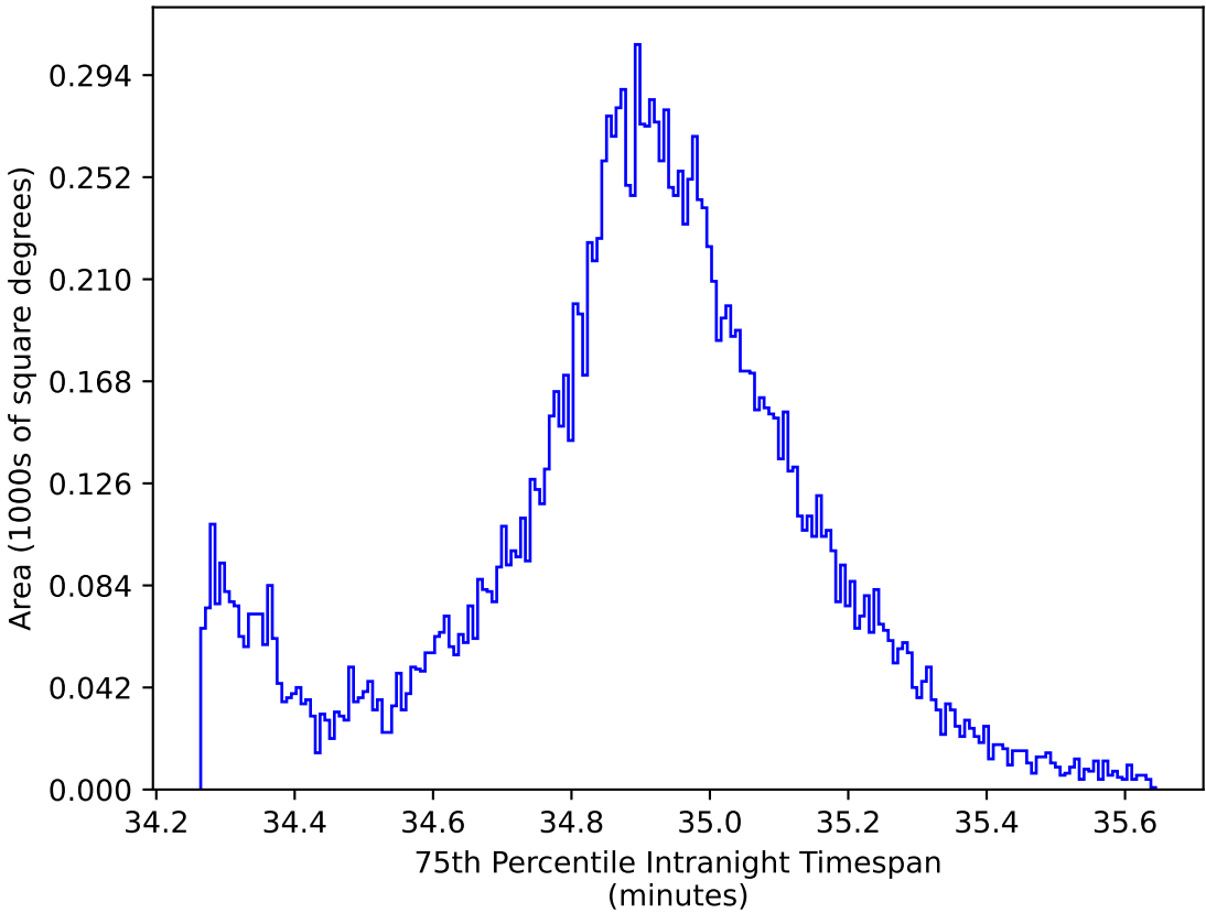
too_elab_r8_d3_giz_v3.4_10yrs WFD: 75th Percentile Intranight Timespan
