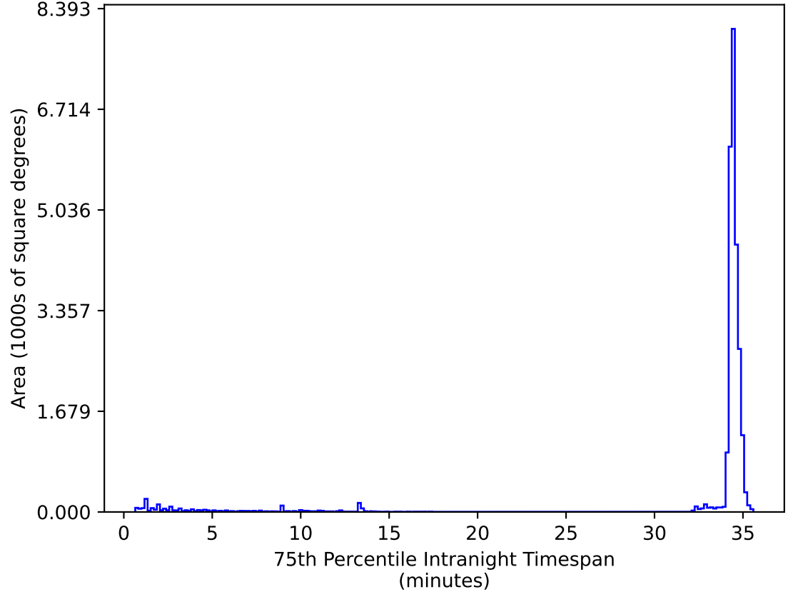
too_elab_r8_d3_giz_v3.4_10yrs All sky zy bands: 75th Percentile Intranight Timespan
