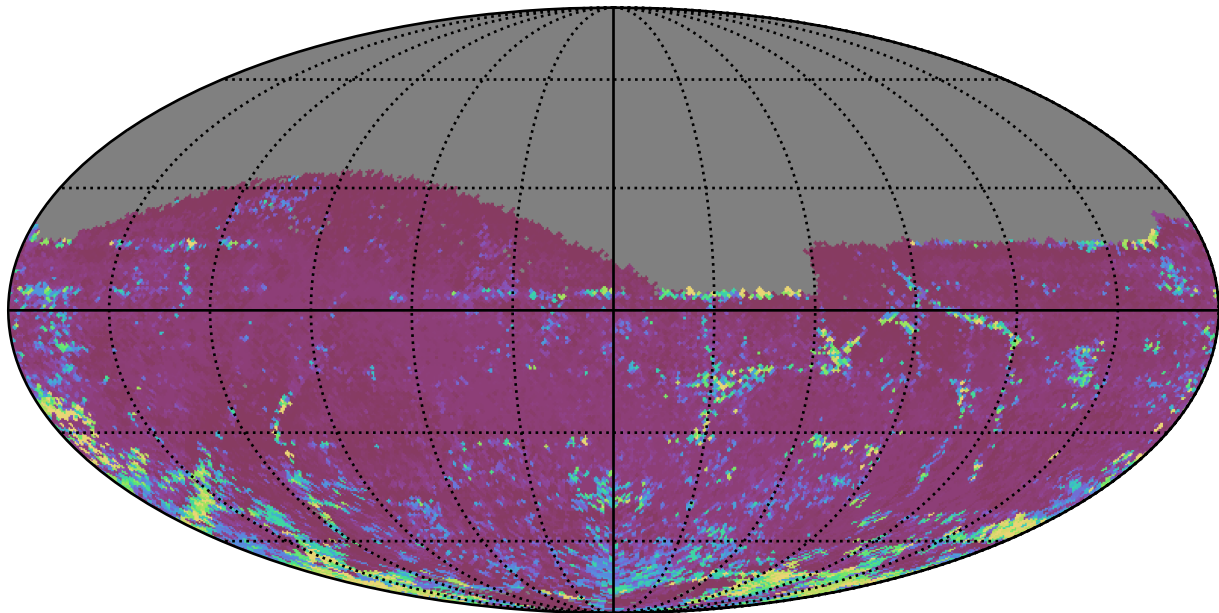
too_elab_r8_d3_giz_v3.4_10yrs All sky z band: 75th Percentile Intranight Timespan
