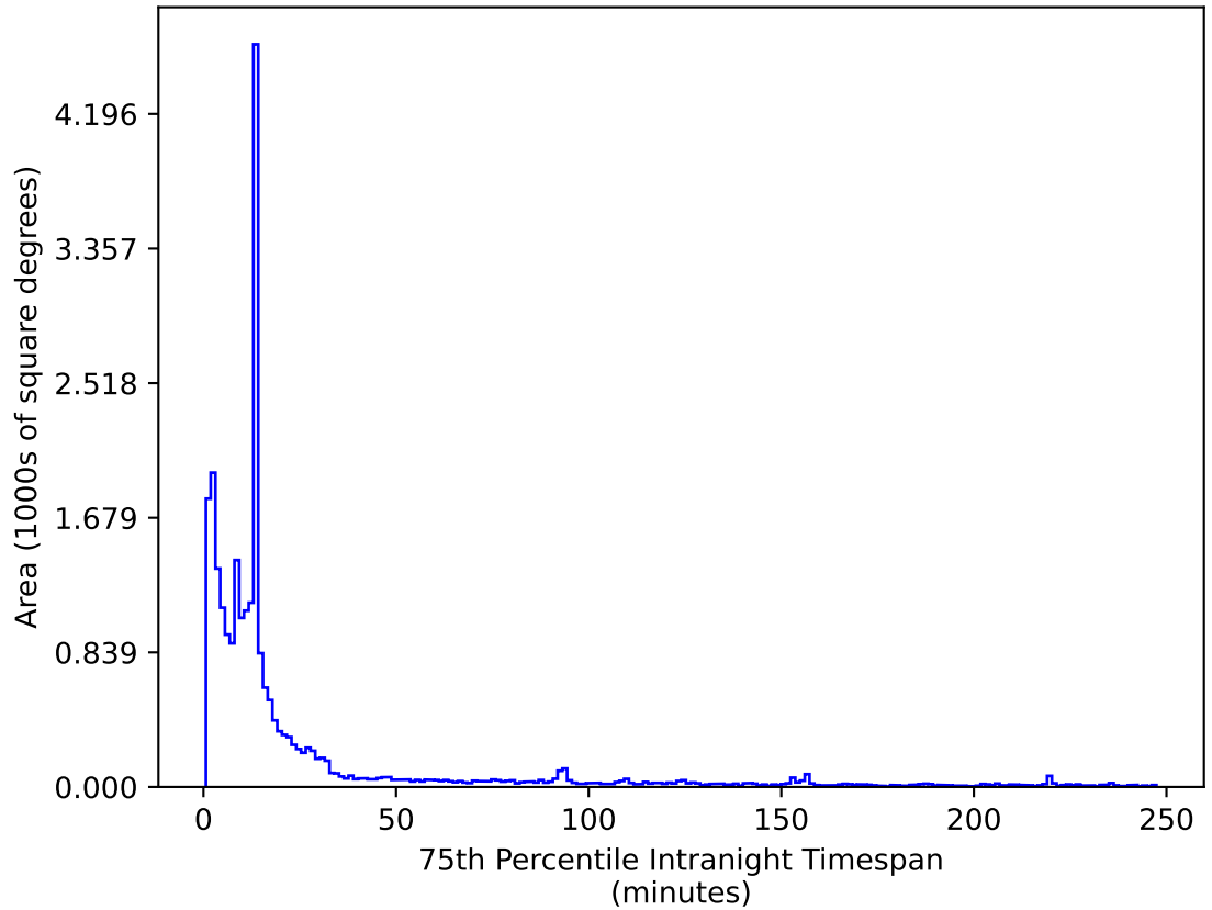
too_elab_r8_d3_giz_v3.4_10yrs All sky z band: 75th Percentile Intranight Timespan
